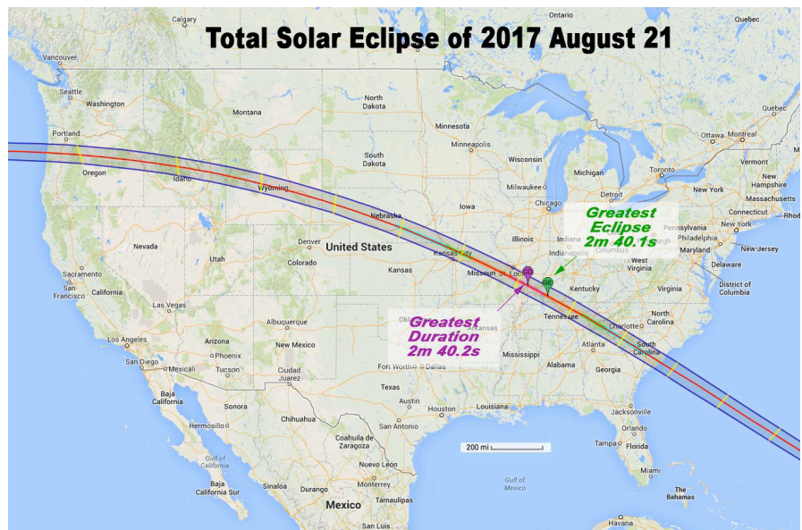
Path of the total solar eclipse over the U.S., map from NASA - Total Solar Eclipse
